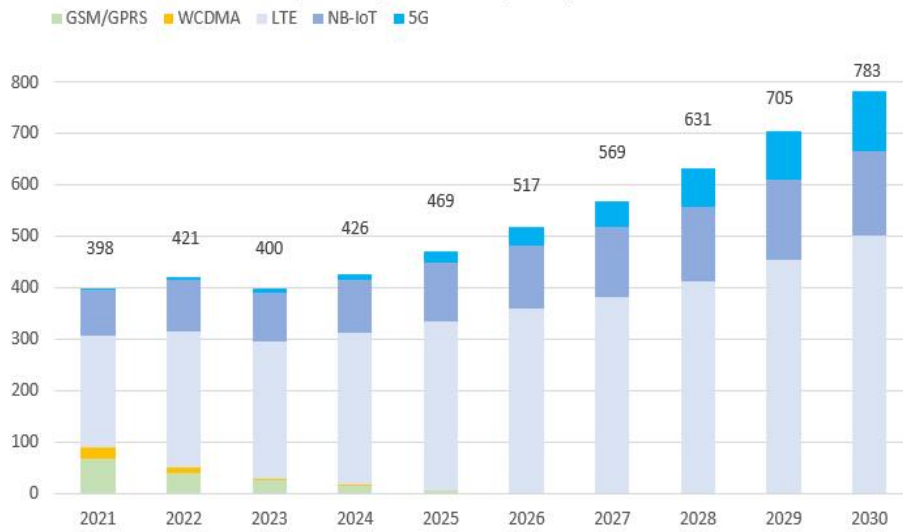
Total Cellular M2M Module Shipments by Air Interface (million)
